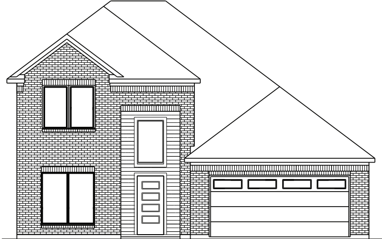
ELEVATION S
